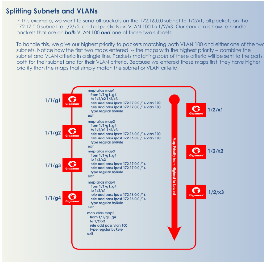
Figure 45 Sending Subnets and VLANs to Different Ports
