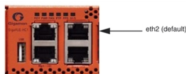
Figure 90 Stack Port Location on GigaVUE-HC1 Front
