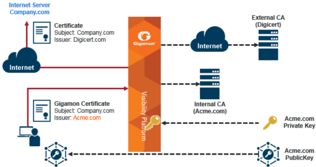
Figure 85 Outbound Deployment of Inline SSL Decryption
