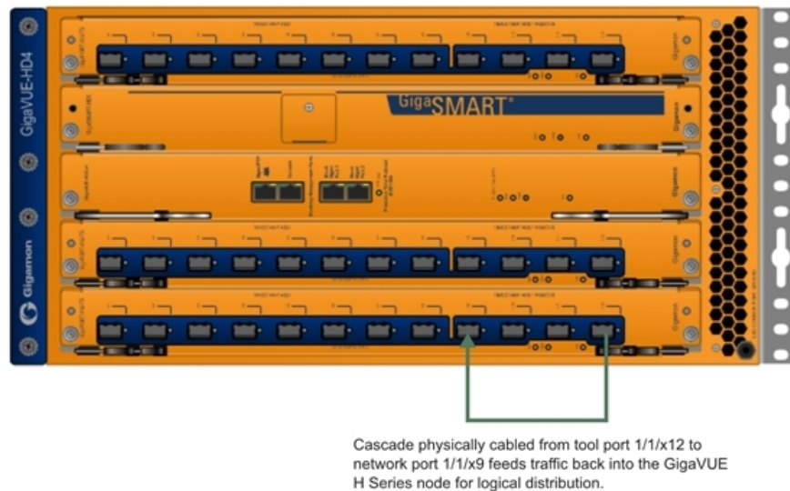
Figure 154 Cascade Physically Cabled from Tool to Network Port
