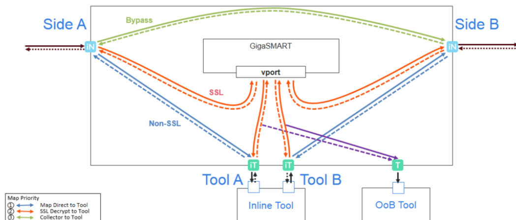
Figure 87 Packet Flow for Inline SSL Decryption
