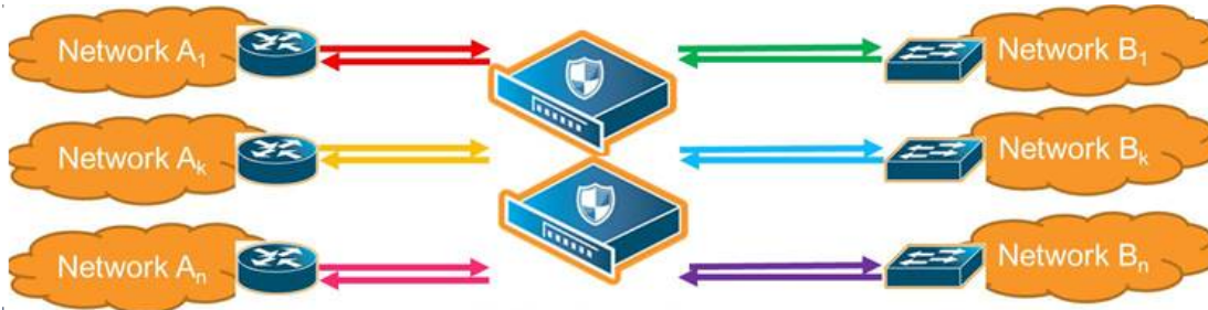
Figure 87 Inline Tool Inserted in Multiple NetA-NetB Links
