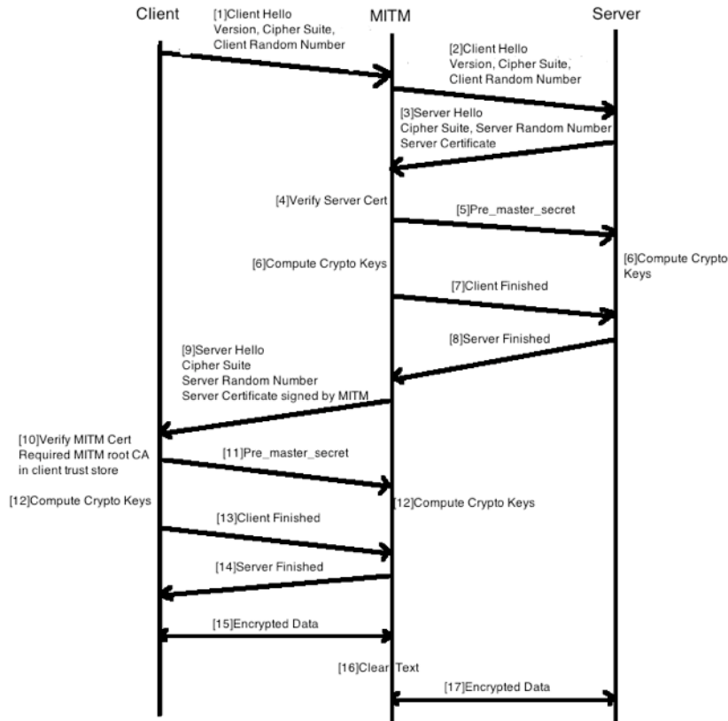
Figure 75 Man-in-the-Middle SSL Handshake
