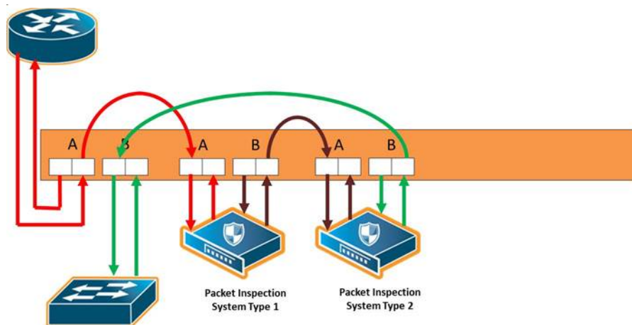
Figure 77 Inline Tool Series
