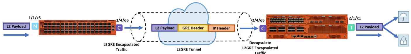
Figure 31 L2GRE Tunnel Encapsulation and Decapsulation
