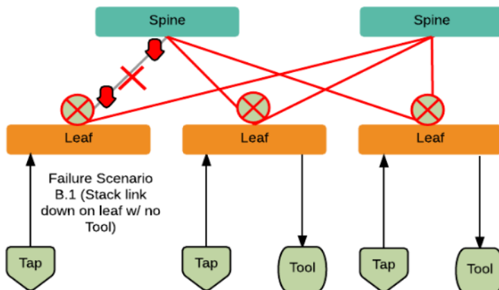
Figure 31 Stack Link Failure on Leaf (TAP Connected)
