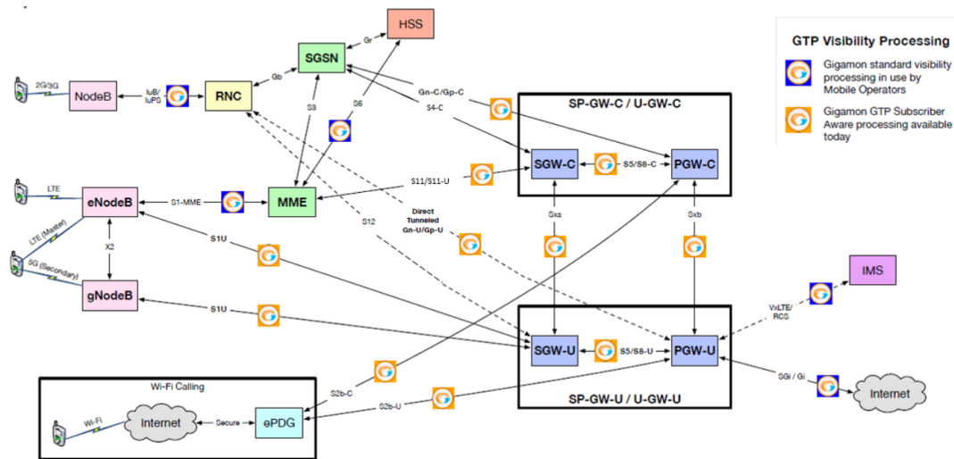
Figure 5 3GPP CUPS Network topology
