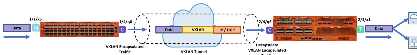
Figure 32 VXLAN Tunnel Encapsulation and Decapsulation
