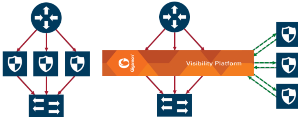
Figure 82 Multiple Inline Tool Arrangement
