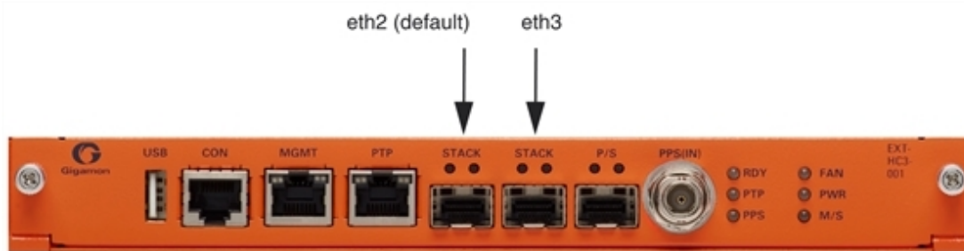
Figure 89 Stack Port Location on GigaVUE-HC3 Front
