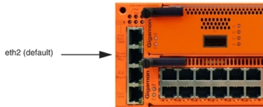
Figure 88 Stack Port Location on GigaVUE-HC2 Front
