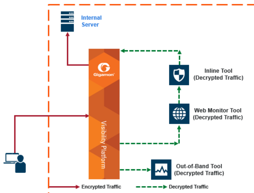
Figure 84 Inbound Deployment of Inline SSL Decryption
