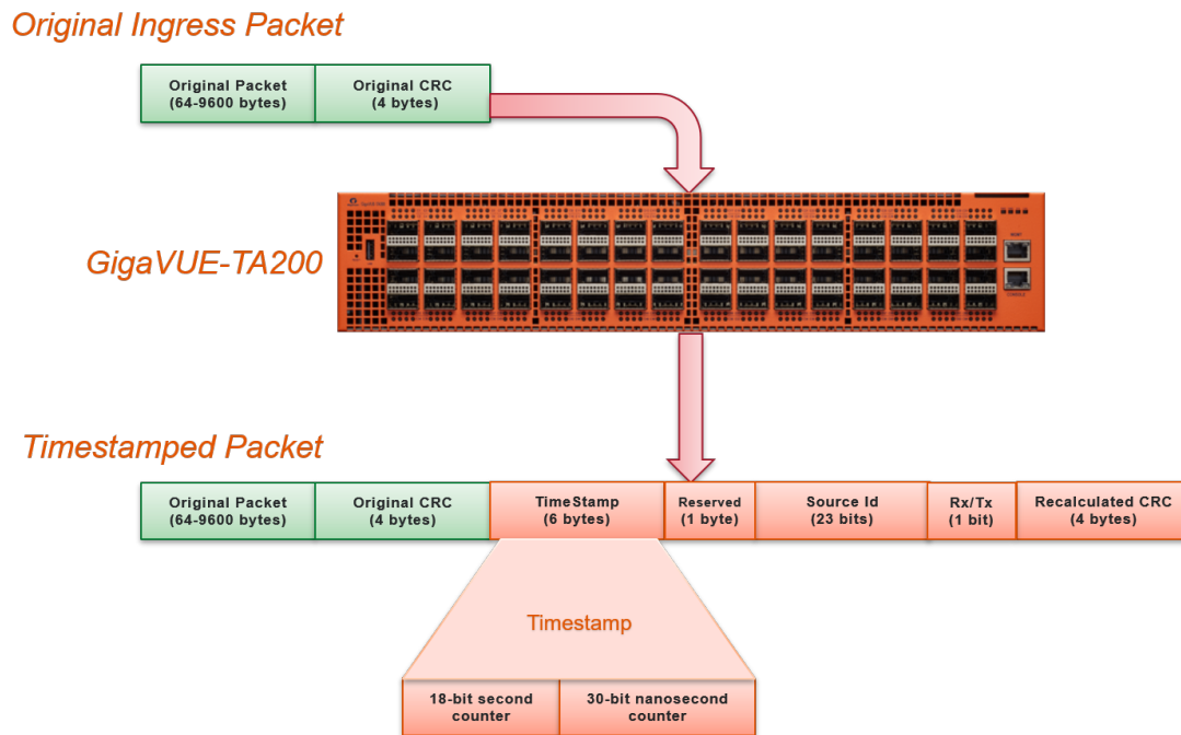
Figure 121 Timestamp Format
