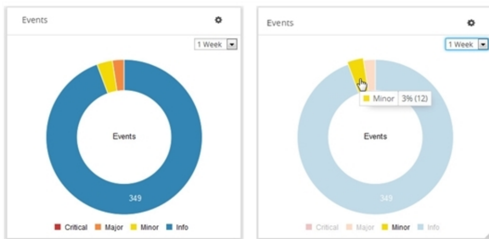
Figure 46 Events Widget
