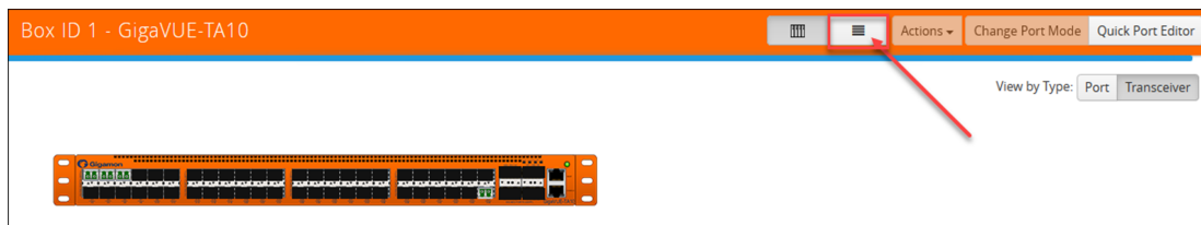
Figure 135 Chassis Screen
