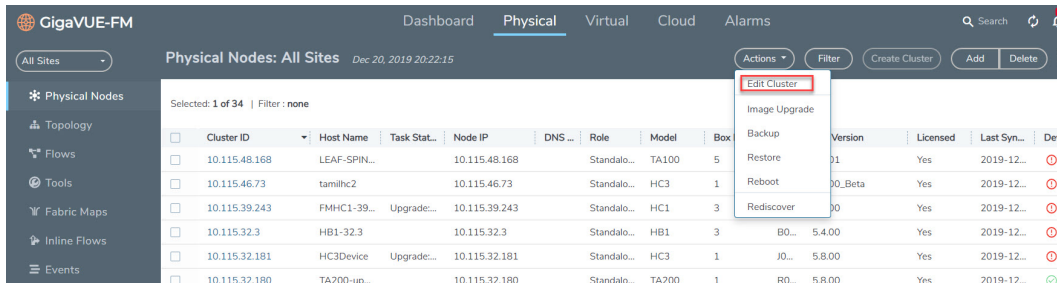
Figure 48 Edit cluster
