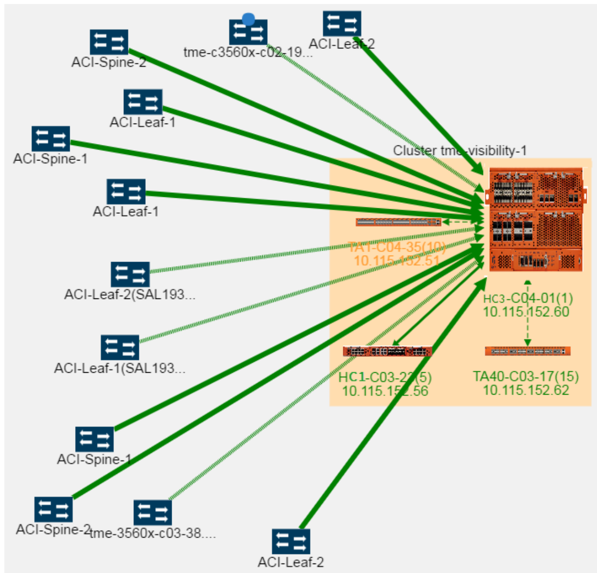
Figure 86 Aligning Neighbors
