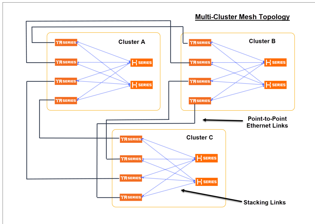
Figure 130 Multi-Cluster Mesh
