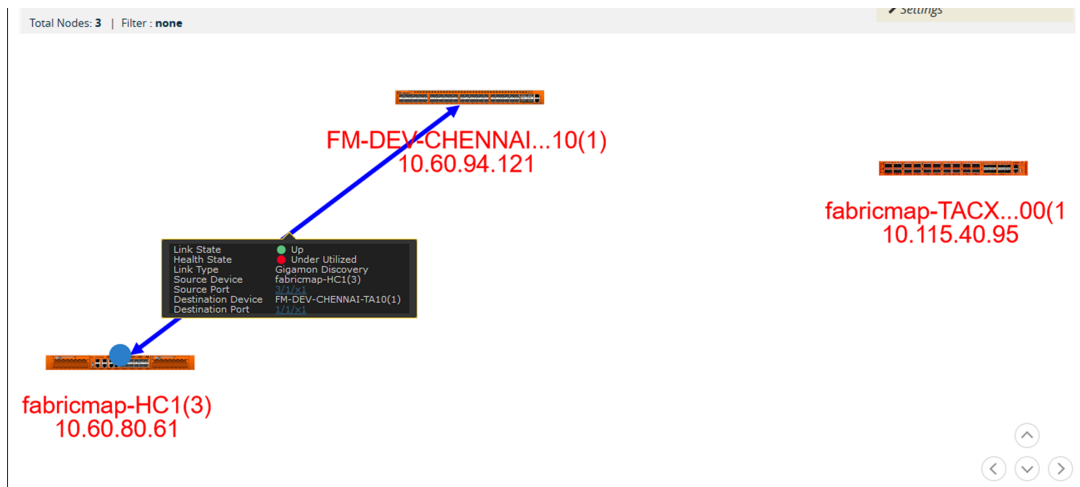
Figure 133 Connecting Devices
