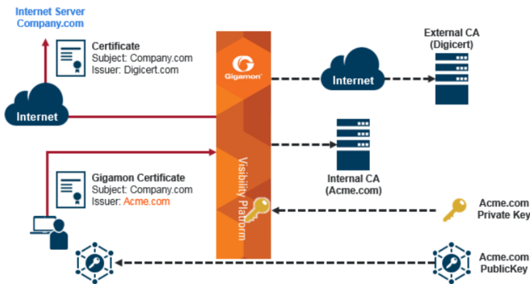
Figure 77 Outbound Deployment of Inline SSL Decryption
